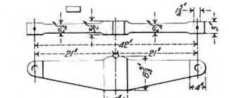
Figs. 1670-1671. Driver Equalizer for Atlantic (4-1-2) Locomotive. American Locomotive Co.
